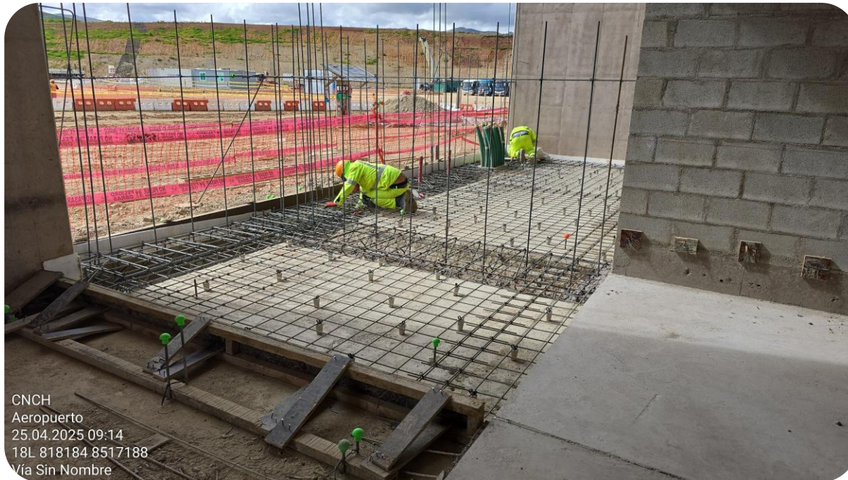
Losa 53 / Slab 53
